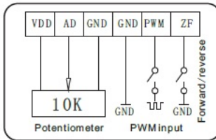
Fig13 External control wiring
