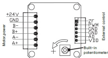
Fig9 Terminal definition
