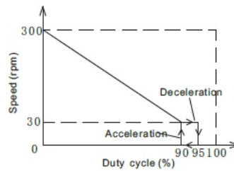
Fig11 Speed graph adjusted by PWM signal
