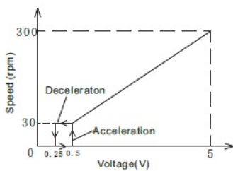
Fig10 Speed graph adjusted by external potentiometer
