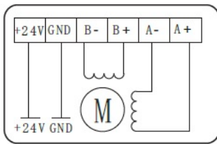
Fig12 Motor&power wiring
