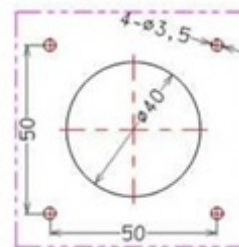
Mounting hole drawing
