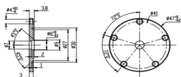
flange drawing
